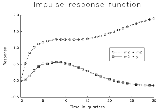
Figure 2: M2 and output responses from M2 VAR of figure 1, plotted on same scale.
