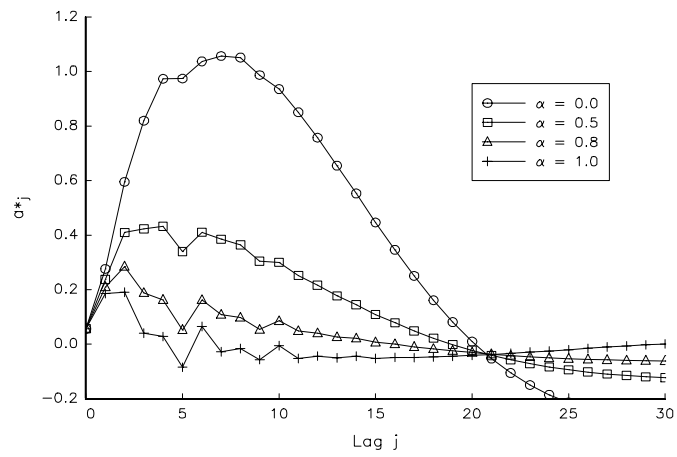
a^*(L) , sticky price model, M2 VAR
