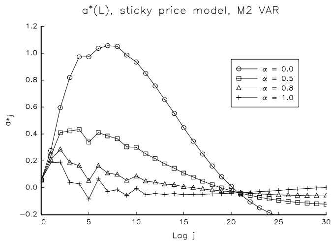
Figure 4: Lag polynomial a^*(L) inferred from m2 impulse-response function using sticky price model. \alpha = price stickiness parameter.
