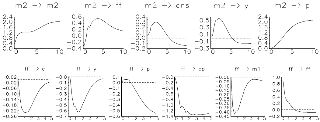
Figure 1: Responses to monetary shocks in two VARs. Horizontal axis in years, variables are 100*logs except ff in percent. Top panel: response to M2 shocks . Bottom panel: response to ff shocks. See the appendix for details on the VAR specification and estimation
