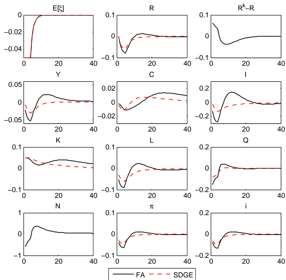
Figure 6: Impulse responses to unrealized news shocks in a model with financial accelerator (FA) and without it (SDGE)
