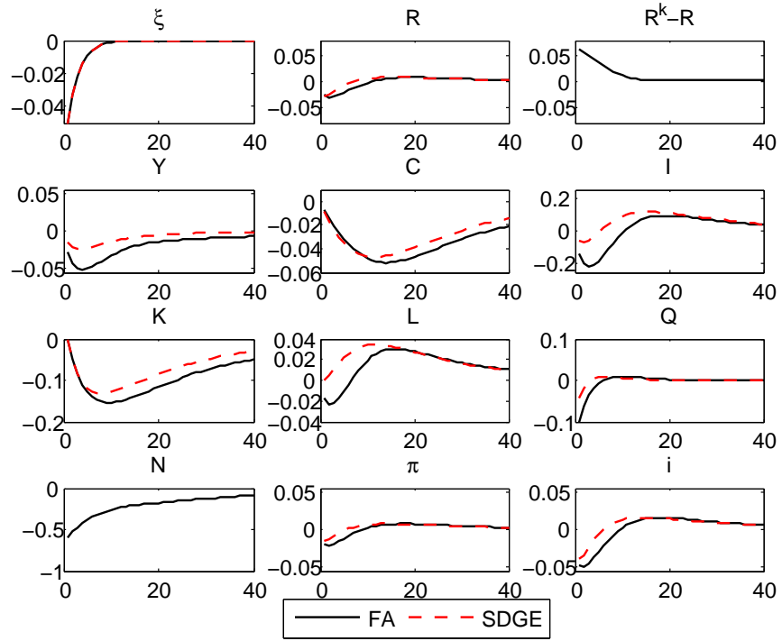
Figure 2: Responses to a Capital Quality Shock
