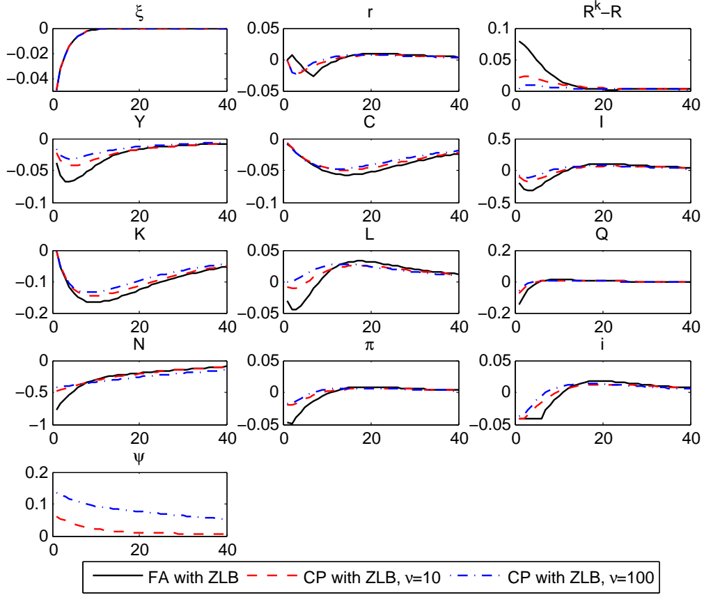
Figure 5: Impulse responses to the capital quality shock with the zero lower bound (ZLB) with and without credit policy
