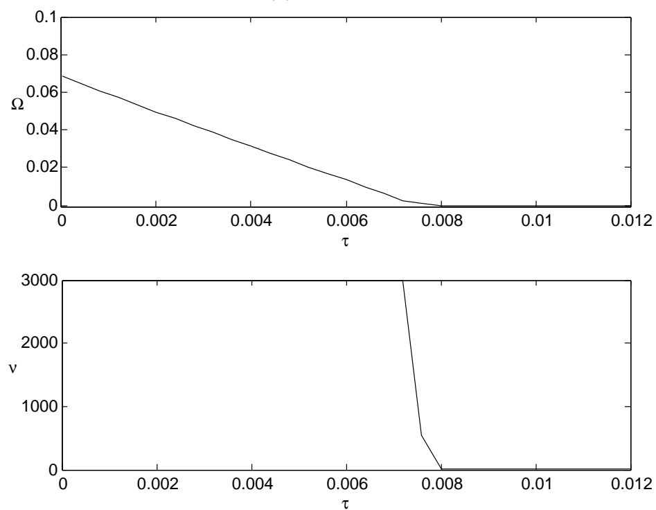
Figure 7: One year consumption equivalent net welfare gains from optimal credit policy ( \Omega ) and optimal credit policy coefficient ( \nu ) as a function of efficiency costs \tau
